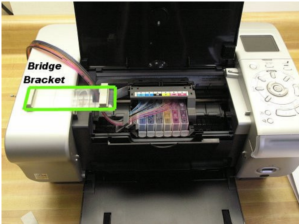
Bridge Bracket and beige clip installation
